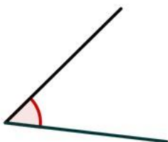
spitzer Winkel
